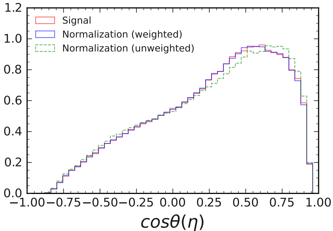
Distributions for D^+ \rightarrow \eta_{3\pi} K^+ and D^+ \rightarrow \eta_{3\pi} \pi^+
