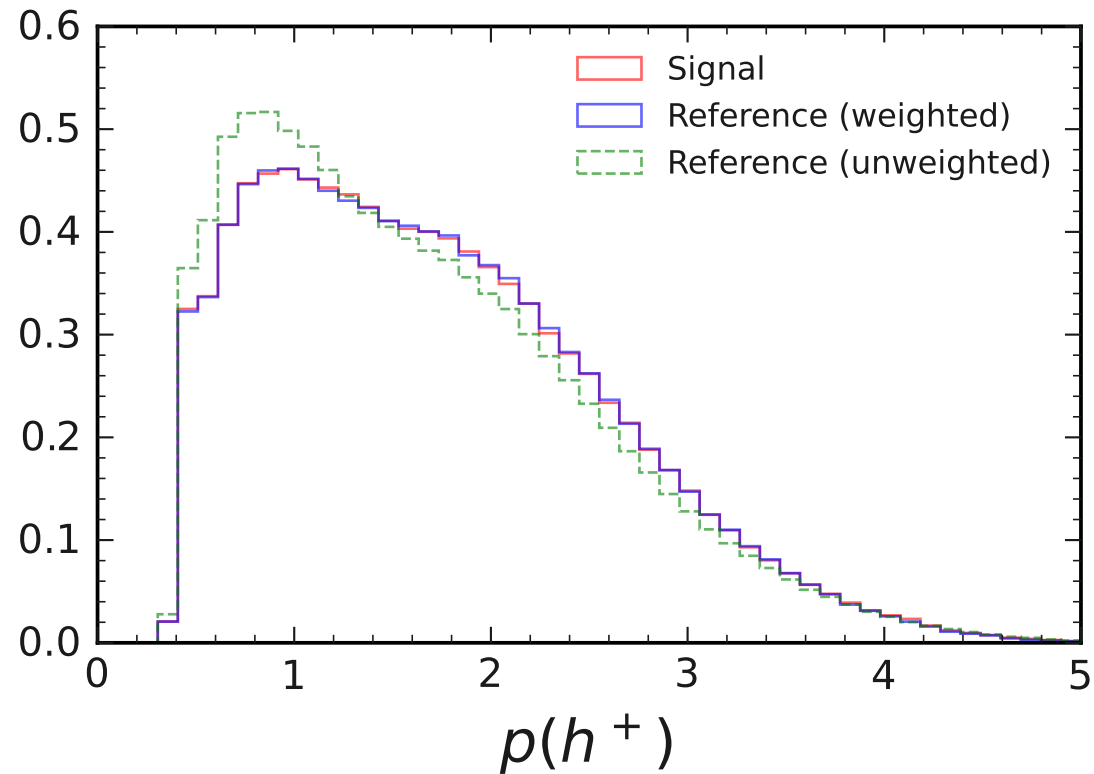
Normalized Distributions for D_s^+ \rightarrow \eta_{\gamma\gamma} \pi^+ and D^+ \rightarrow K_S^0 \pi^+
