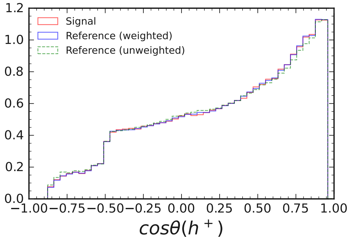
Normalized Distributions for D_s^+ \rightarrow \eta_{\gamma\gamma} \pi^+ and D^+ \rightarrow K_S^0 \pi^+
