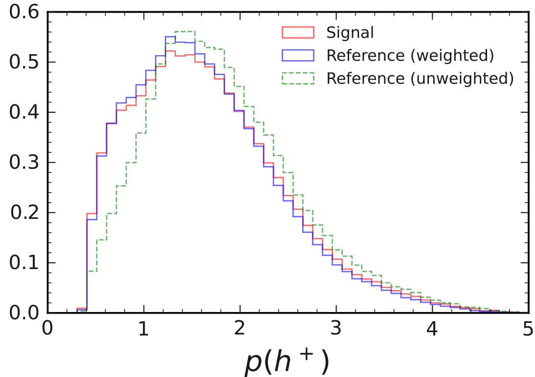
Normalized Distributions for D_s^+ \rightarrow \eta_{\gamma\gamma} K^+ and D_s^+ \rightarrow K_S^0 K^+
