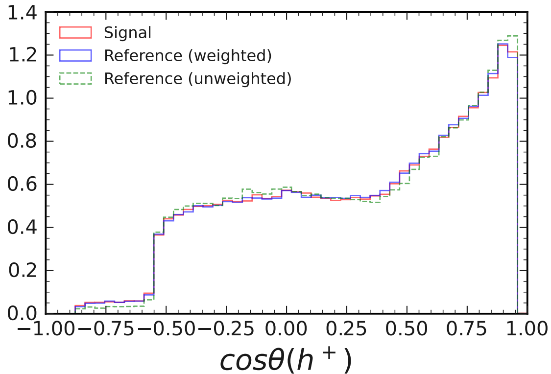
Normalized Distributions for D_s^+ \rightarrow \eta_{\gamma\gamma} K^+ and D_s^+ \rightarrow K_S^0 K^+
