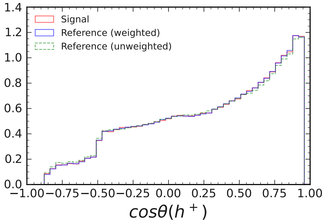
Normalized Distributions for D_s^+ \rightarrow \eta_{3\pi} \pi^+ and D^+ \rightarrow K_S^0 \pi^+
