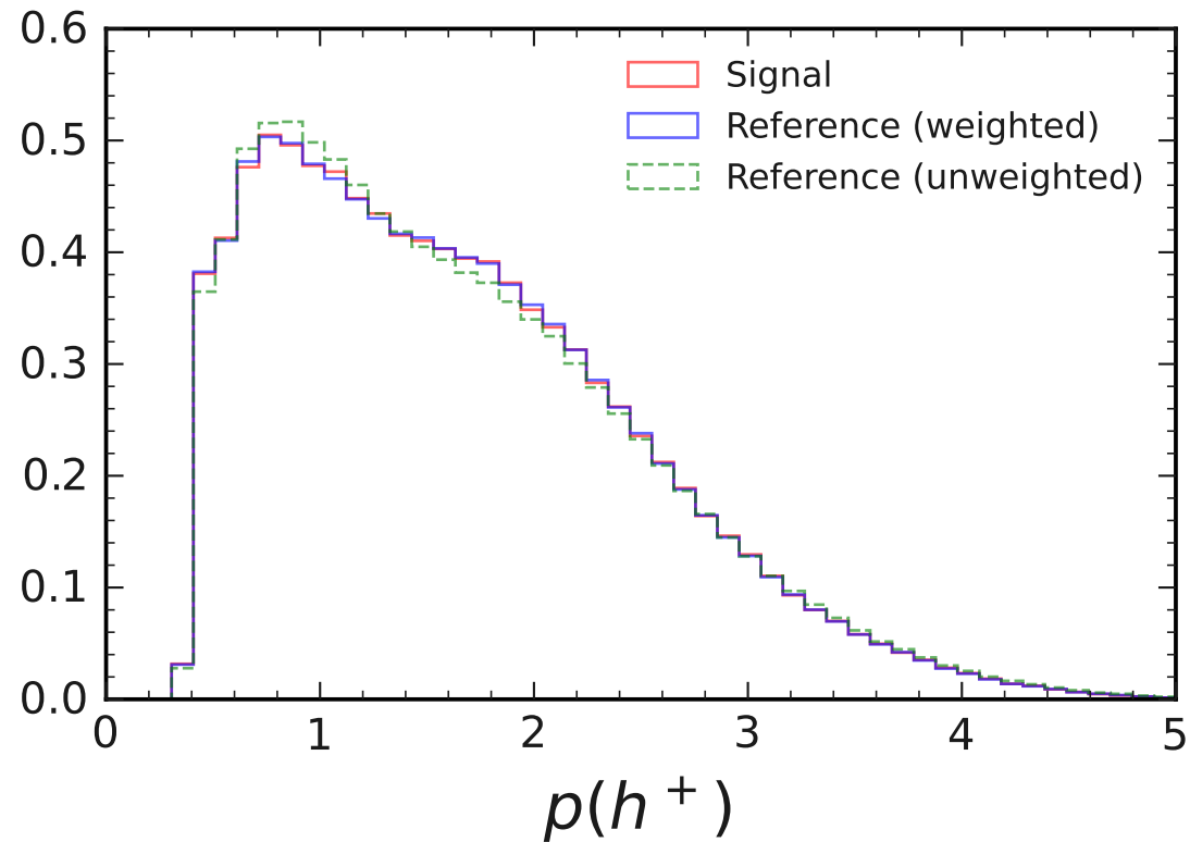
Normalized Distributions for D^+ \rightarrow \eta_{\gamma\gamma} \pi^+ and D^+ \rightarrow K_S^0 \pi^+
