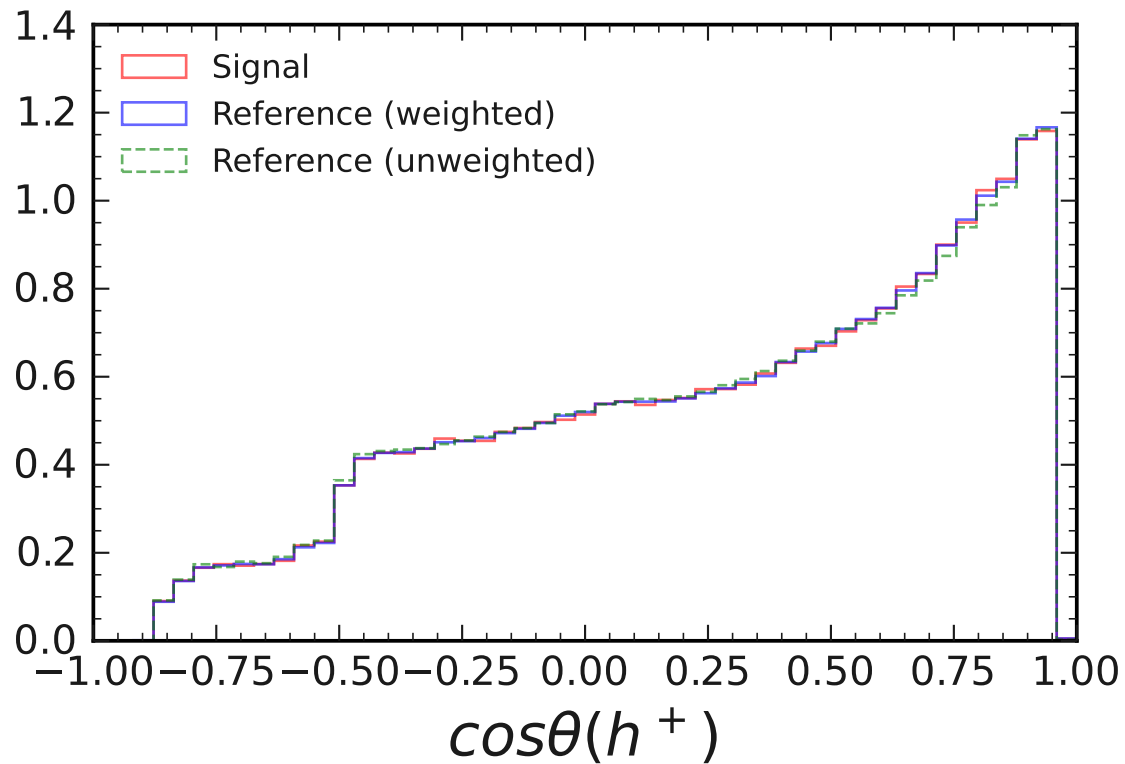
Normalized Distributions for D^+ \rightarrow \eta_{3\pi} \pi^+ and D^+ \rightarrow K_S^0 \pi^+
