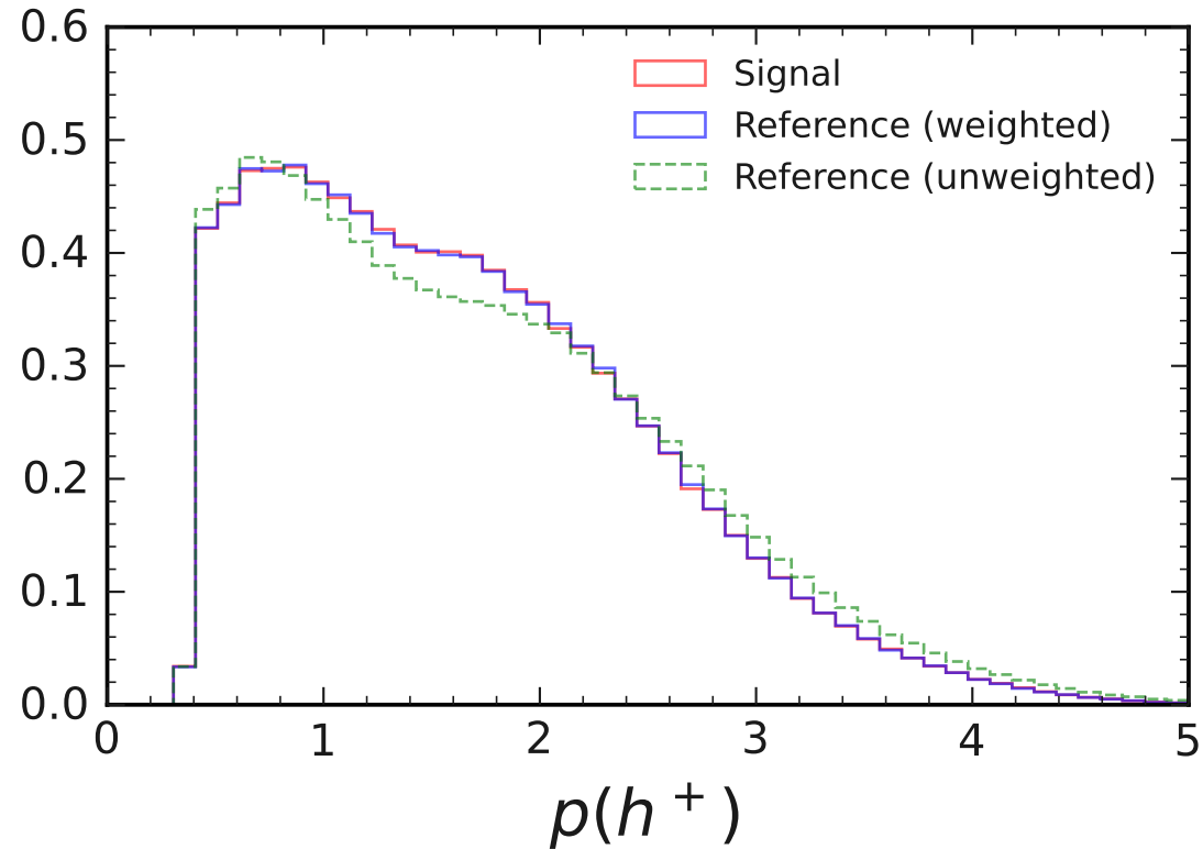
Normalized Distributions for D^+ \rightarrow \eta_{3\pi} \pi^+ and D^+ \rightarrow K_S^0 \pi^+
