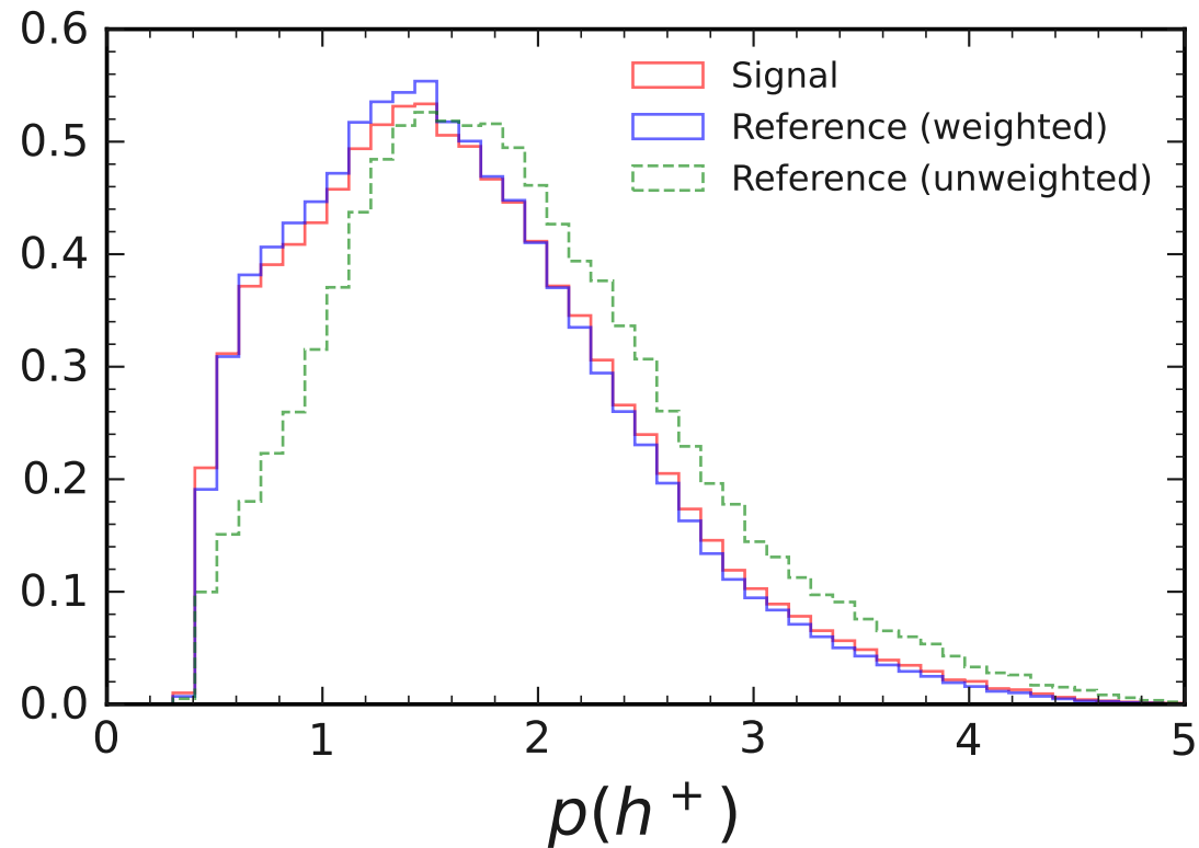
Normalized Distributions for D^+ \rightarrow \eta_{3\pi} K^+ and D_s^+ \rightarrow K_S^0 K^+
