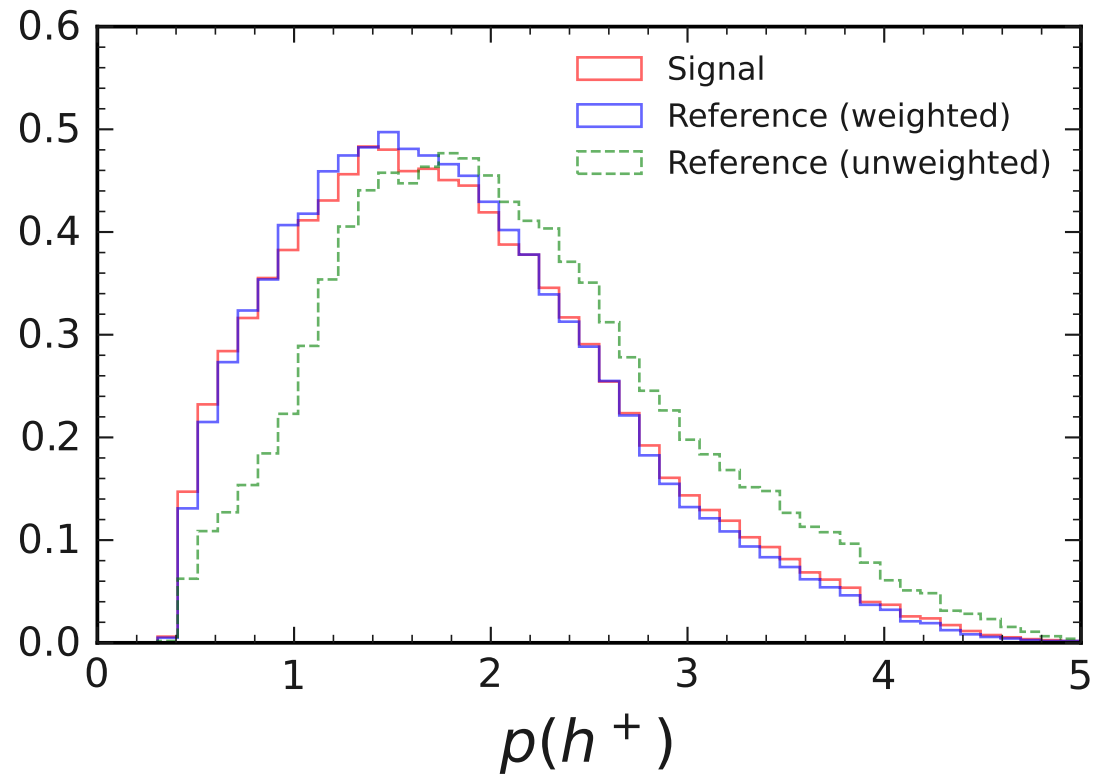
Normalized Distributions for D^+ \rightarrow \eta_{3\pi} K^+ and D_s^+ \rightarrow K_S^0 K^+ in \cos \theta^* > 0
