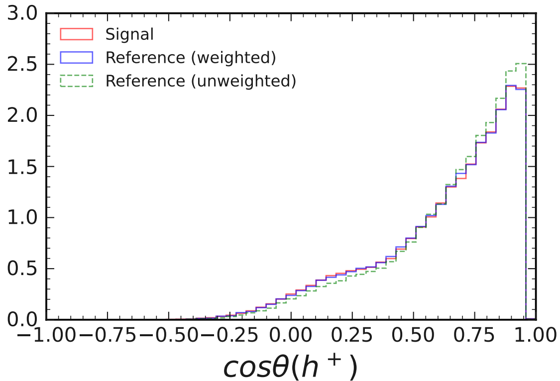
Normalized Distributions for D^+ \rightarrow \eta_{3\pi} K^+ and D_s^+ \rightarrow K_S^0 K^+ in \cos \theta^* > 0
