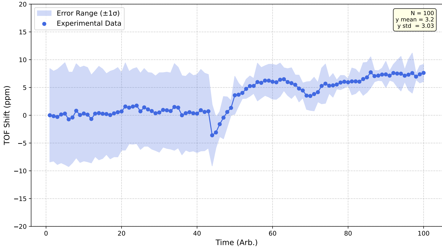
TOF shift as a function of time
