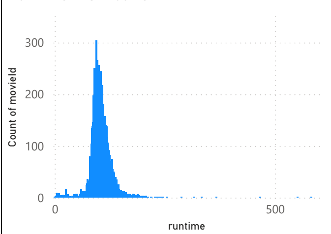
Runtime Distribution
