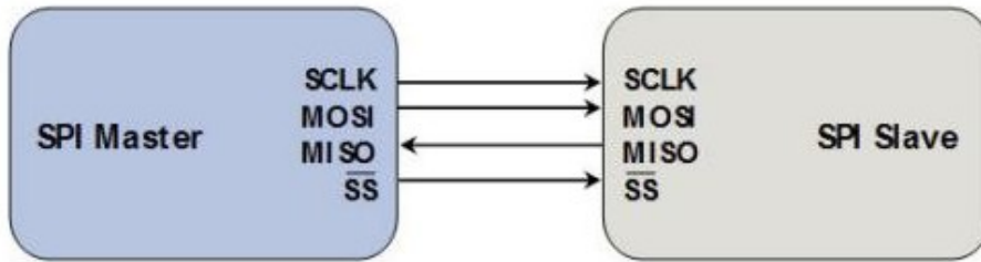
SPI master connected to a single slave (point to point)
