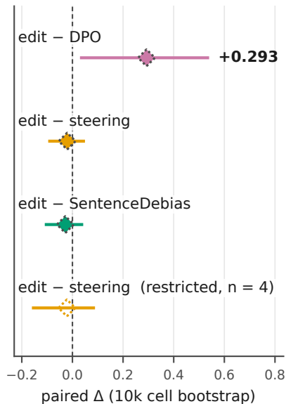
Pooled paired \Delta (n = 8 cells)
