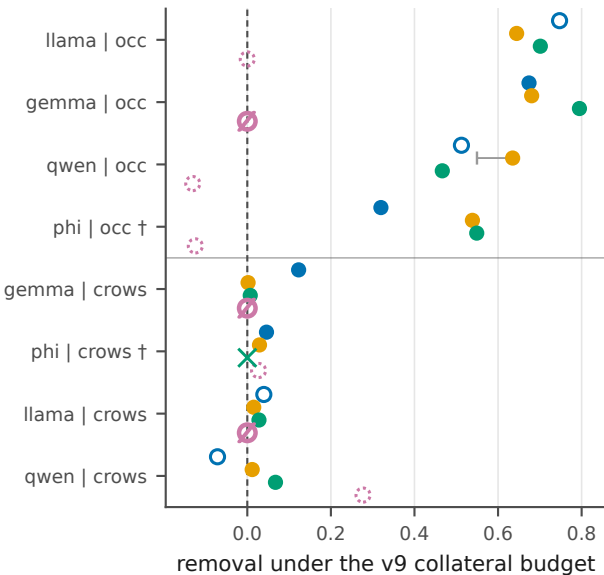
Per-cell removal (8 cells × 4 methods)
