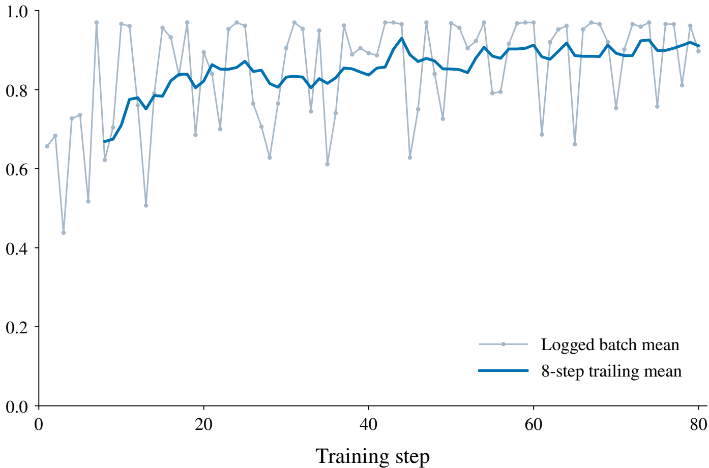
Mean training reward
