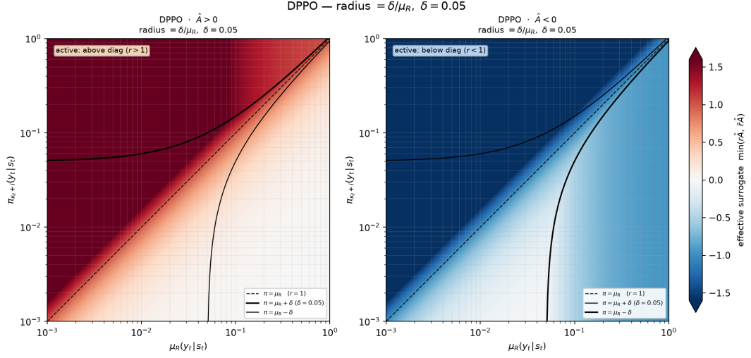
(a) DPPO
