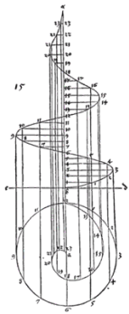
FIG. 359—DIVER'S CALCULATION FOR MAX HELIX FROM A FLAT SPIRAL
