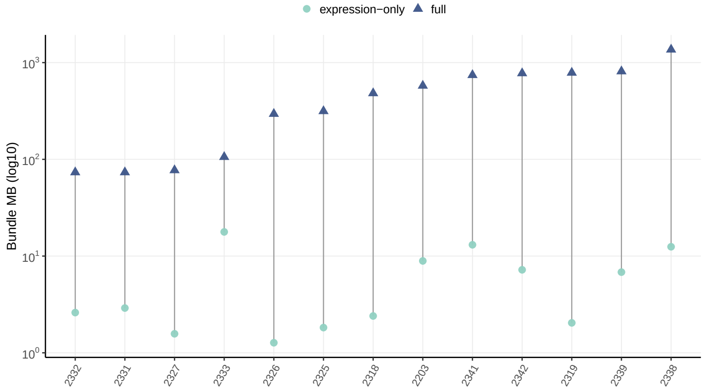
Bundle size: full vs expression-only
