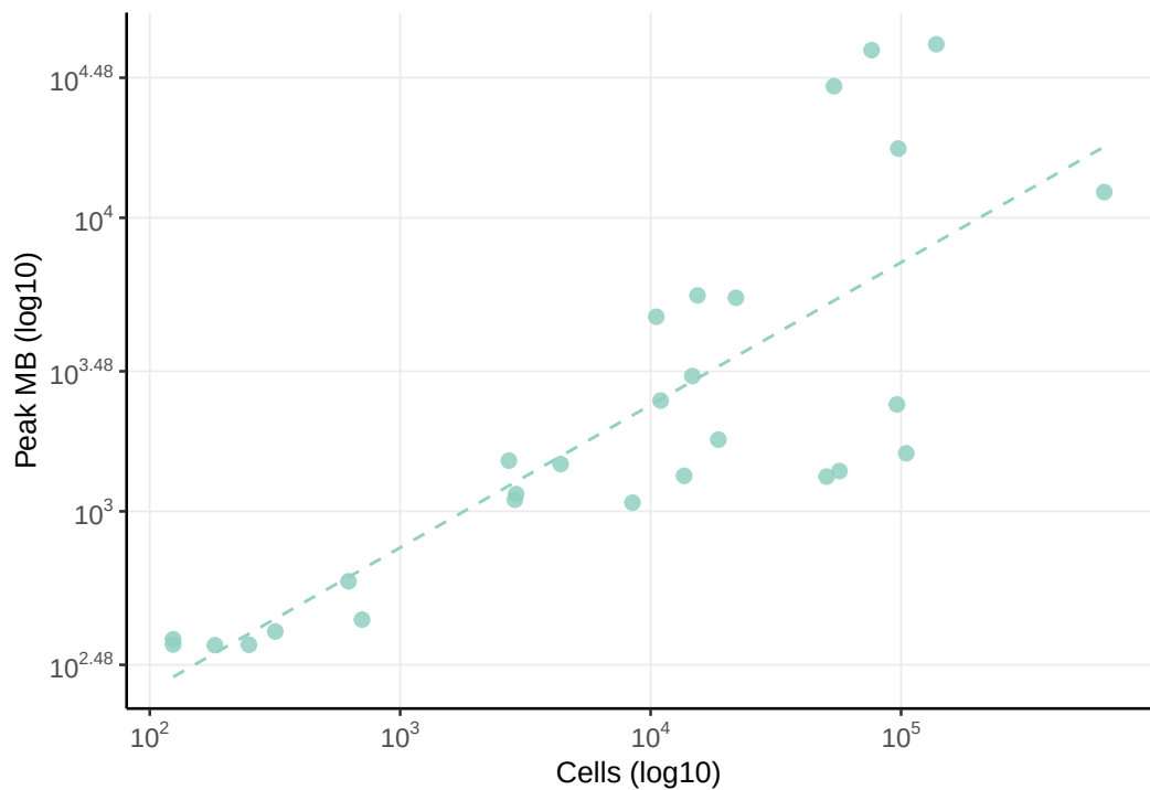
prepare_study() peak memory [expression-only]
