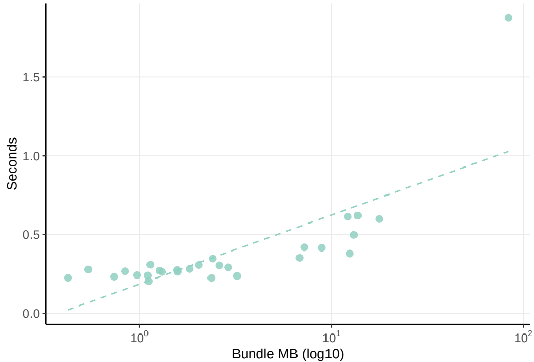
load_study() cold-start latency [expression-only]
