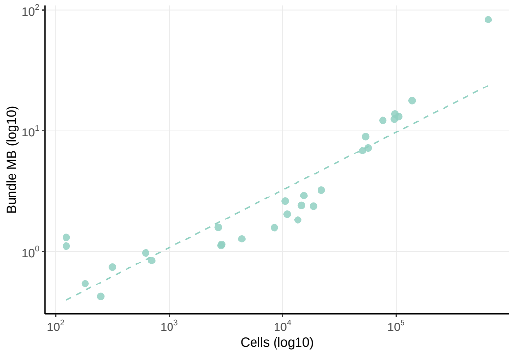
Bundle size [expression-only]
