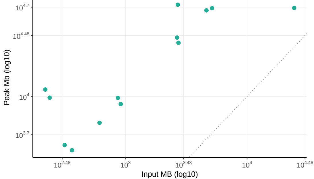
Peak memory vs total input size
