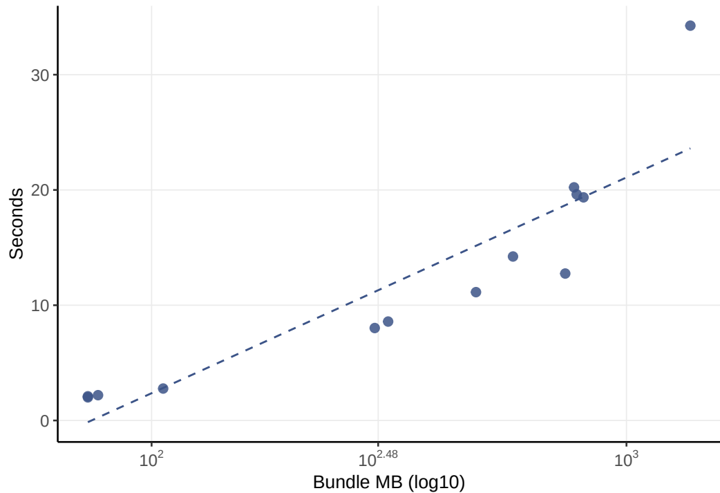
load_study() cold-start latency
