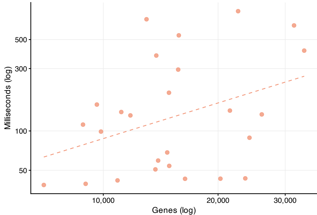
gene_values() fetch latency (median)
