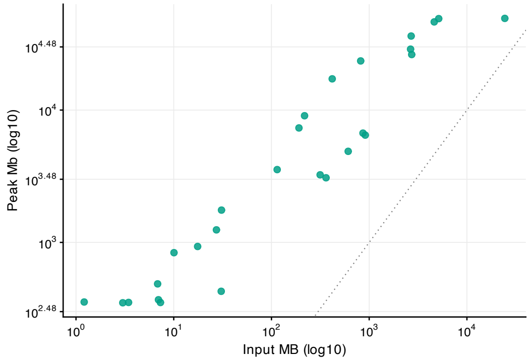
Peak memory vs total input size
