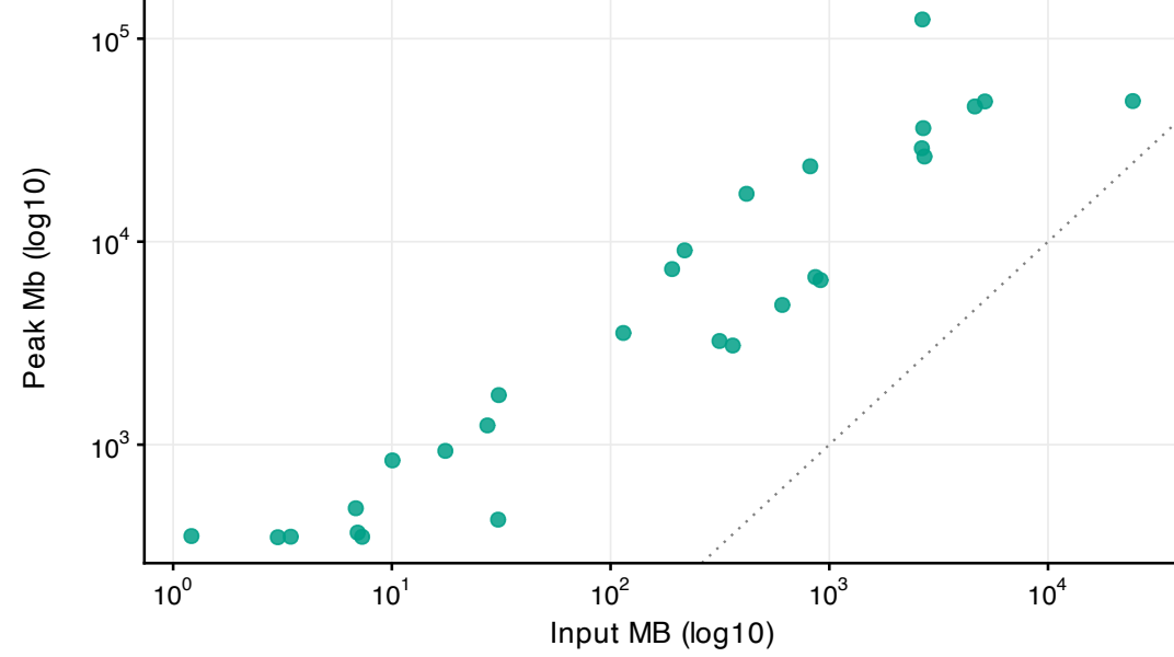
Peak memory vs total input size
