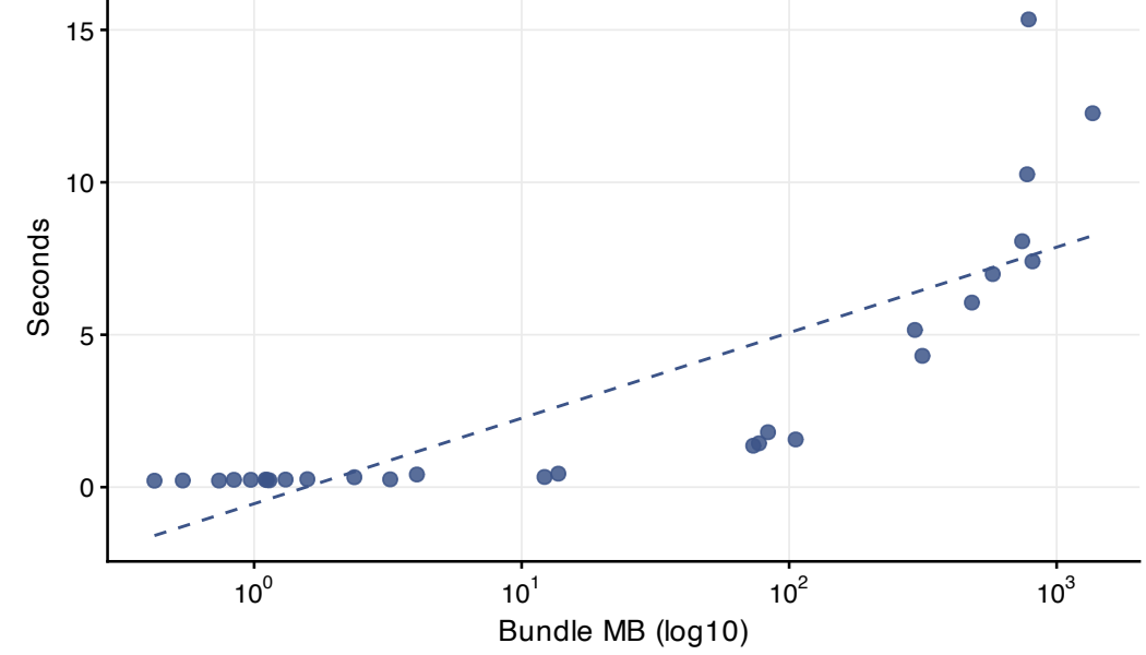
load_study() cold-start latency
