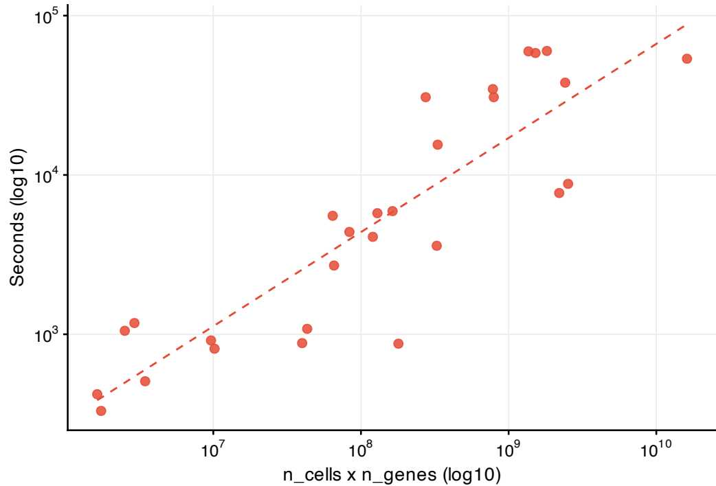
prepare_study() wall time
