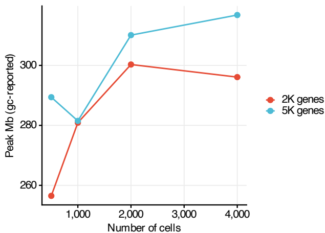
F. prepare_study_data() peak memory
