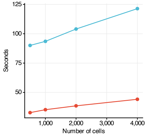
E. prepare_study_data() wall time
