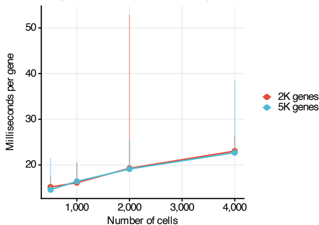
E. prepare_study_data() wall time
