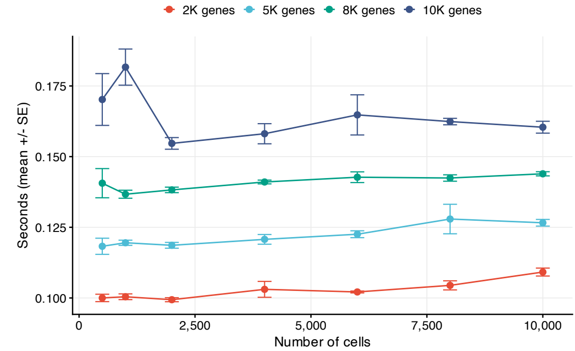
discover_studies() scaling
