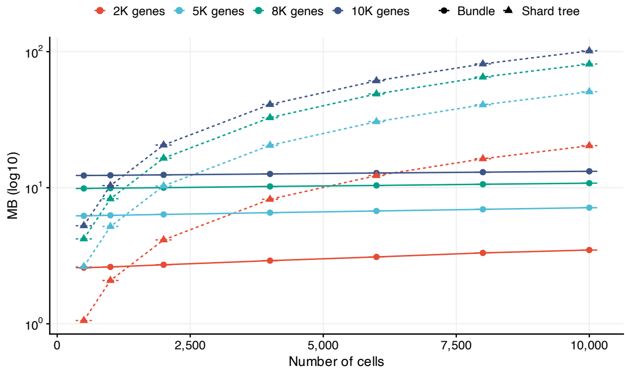
Bundle size vs shard-tree size
