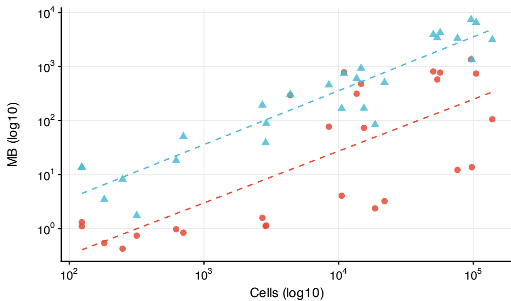
Peak memory vs total input size
