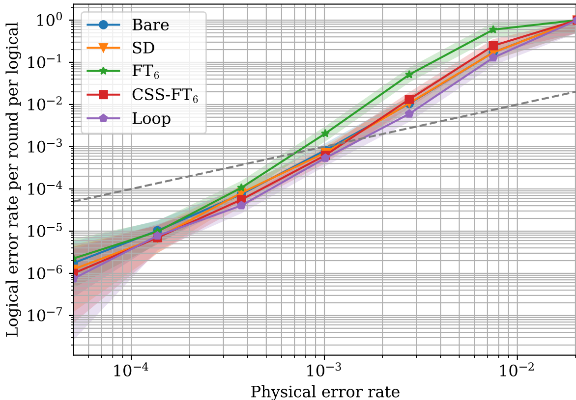
[[30, 8, 4]] with Circuit Noise
