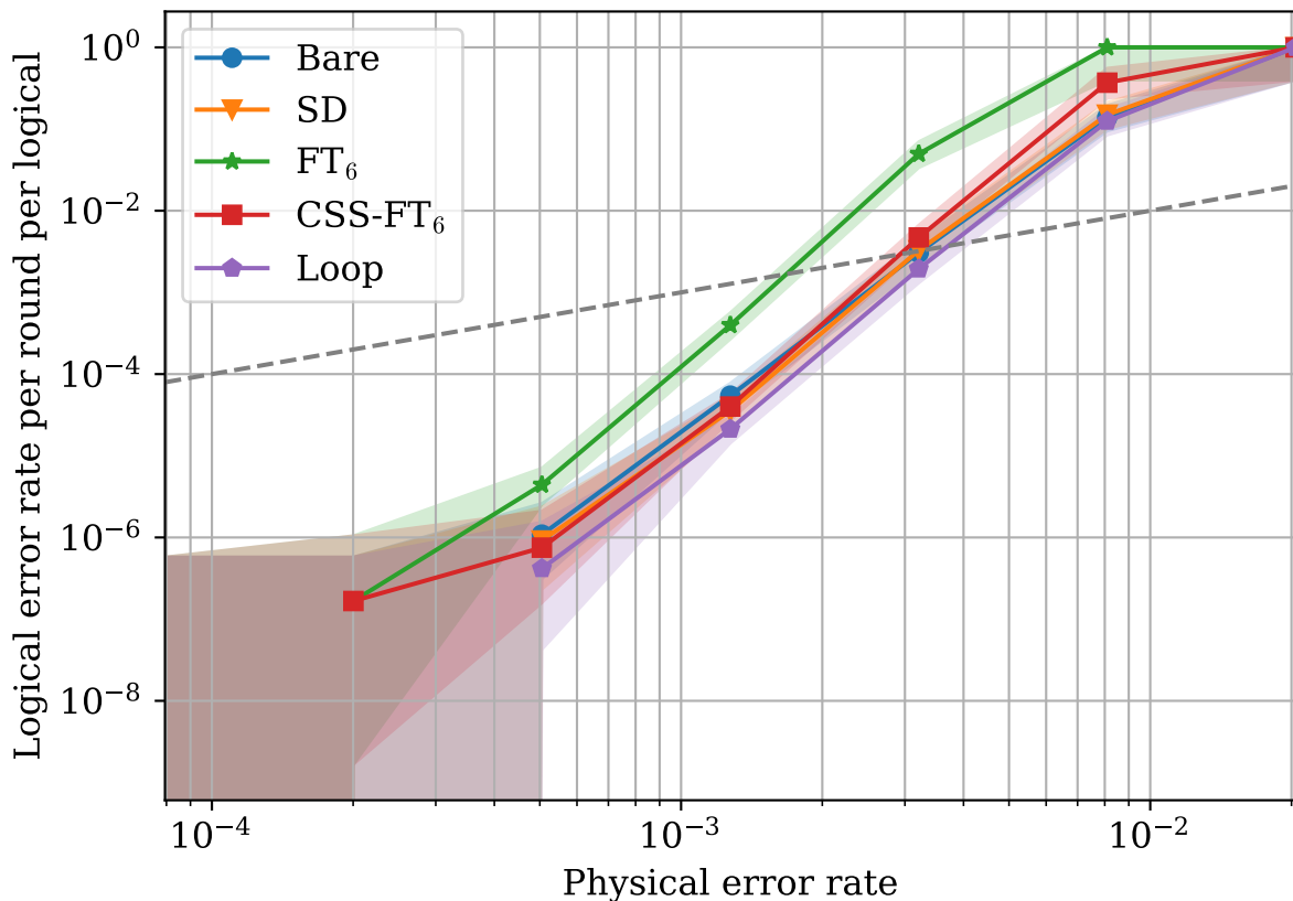
[[36, 6, 6]] with Circuit Noise
