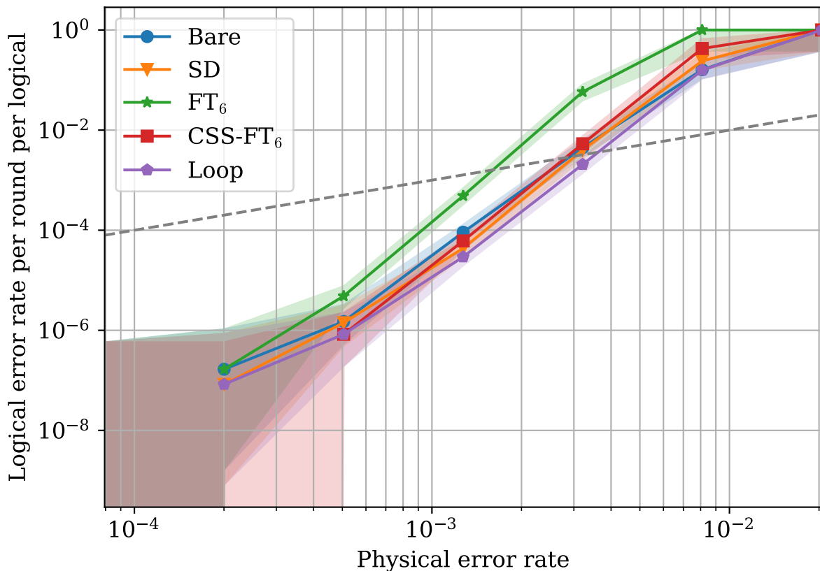
[[48, 8, 6]] with Circuit Noise
