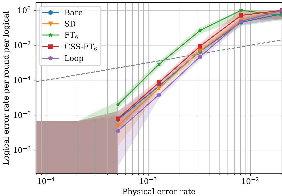
[[48, 4, 8]] with Circuit Noise
