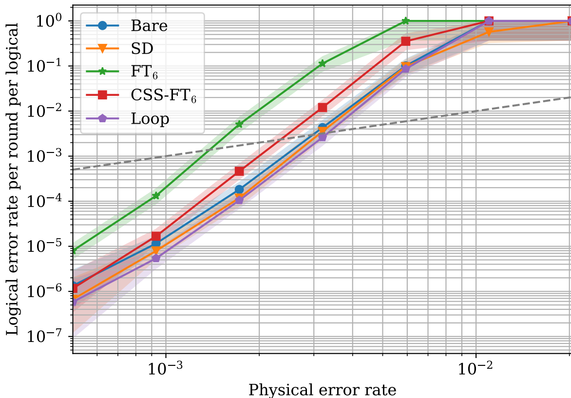
[[72, 12, 6]] with Circuit Noise
