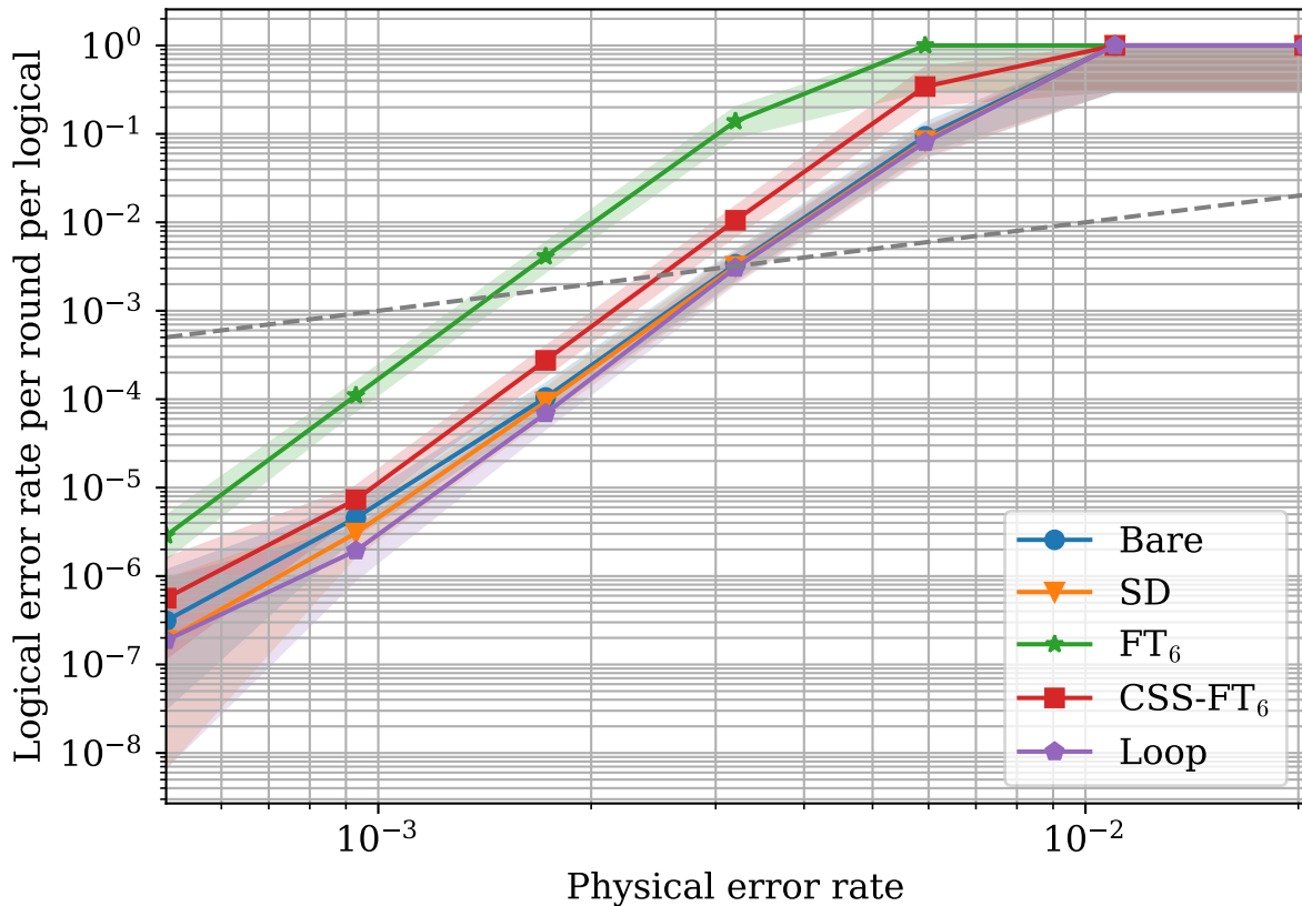
[[72, 8, 8]] with Circuit Noise
