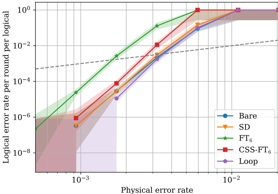
[[85, 8, 9]] with Circuit Noise
