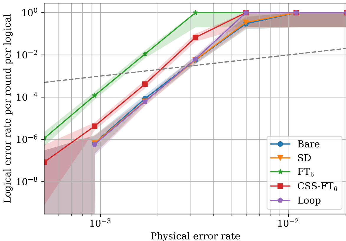
[[144, 12, 12]] with Circuit Noise
