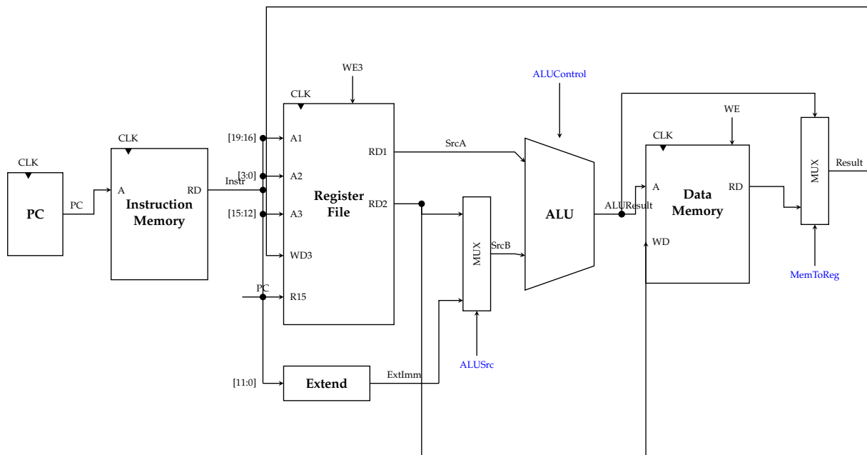
Figure 10.1: Complete single-cycle ARM datapath: PC , Instruction Memory , Register File (with all ports), Extend unit, SrcB multiplexer ( ALUSrc ), ALU , Data Memory , and write-back ( MemToReg ) multiplexer. Blue labels are control signals driven by the Control Unit.
