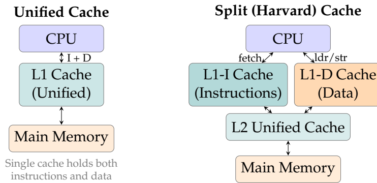
Figure 12.14: Unified cache (left): one cache holds instructions and data. Split (Harvard) cache (right): separate L1 caches for instructions and data allow the CPU to fetch an instruction and load data simultaneously, eliminating the structural hazard seen in the pipelined datapath.
