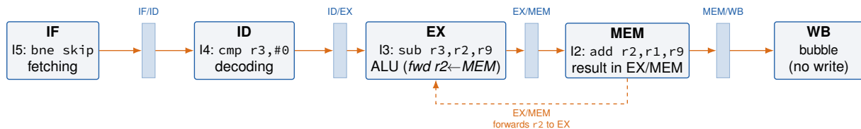
Figure 11.10: Pipeline snapshot at cycle 6. Four instructions occupy four different stages simultaneously: I5 fetching in IF, I4 decoding in ID, I3 executing in EX (receiving I2's result via EX/MEM forwarding), I2 in MEM, and the load-use bubble in WB.
