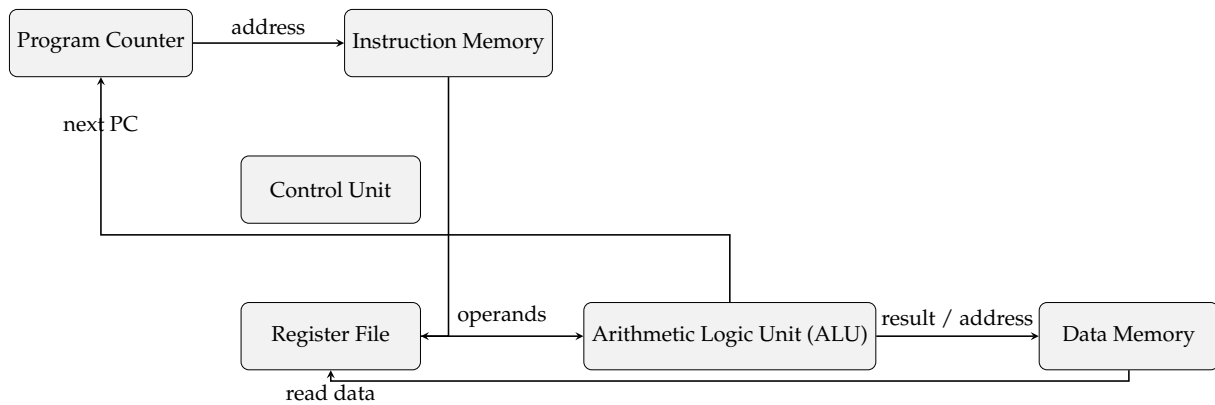
Figure 10.1: Simplified datapath for a single-cycle processor. Each instruction passes through this entire datapath within one clock period.
