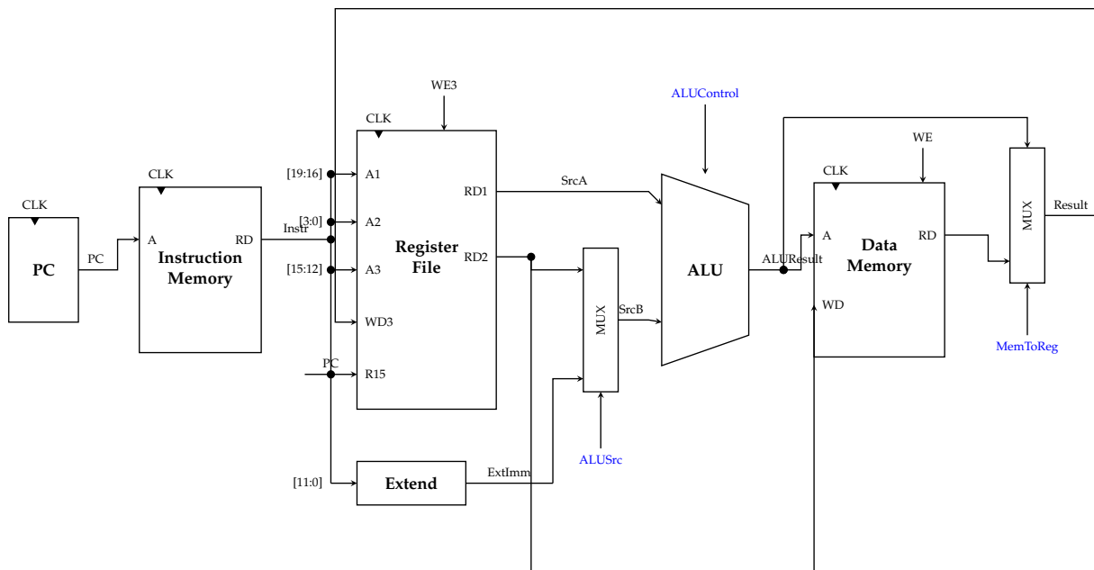
Figure 10.2: Complete single-cycle ARM datapath: PC , Instruction Memory , Register File (with all ports), Extend unit, SrcB multiplexer ( ALUSrc ), ALU , Data Memory , and write-back ( MemToReg ) multiplexer. Blue labels are control signals driven by the Control Unit.
