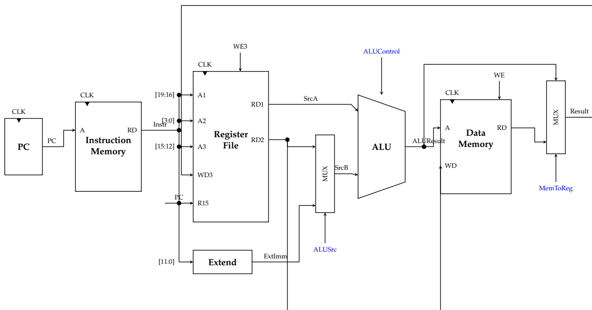
Figure 10.3: Complete single-cycle ARM datapath: PC , Instruction Memory , Register File (with all ports), Extend unit, SrcB multiplexer ( ALUSrc ), ALU , Data Memory , and write-back ( MemToReg ) multiplexer. Blue labels are control signals driven by the Control Unit.
