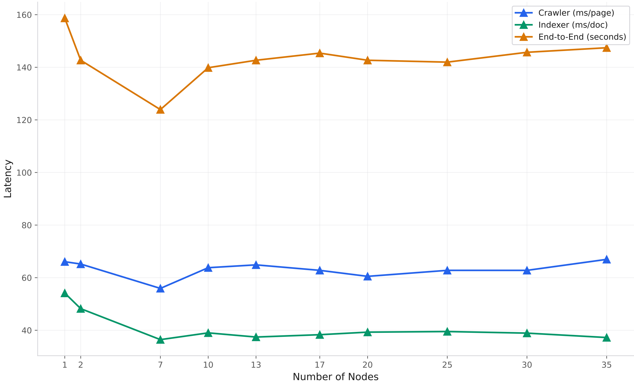
Latency vs. Node Count
