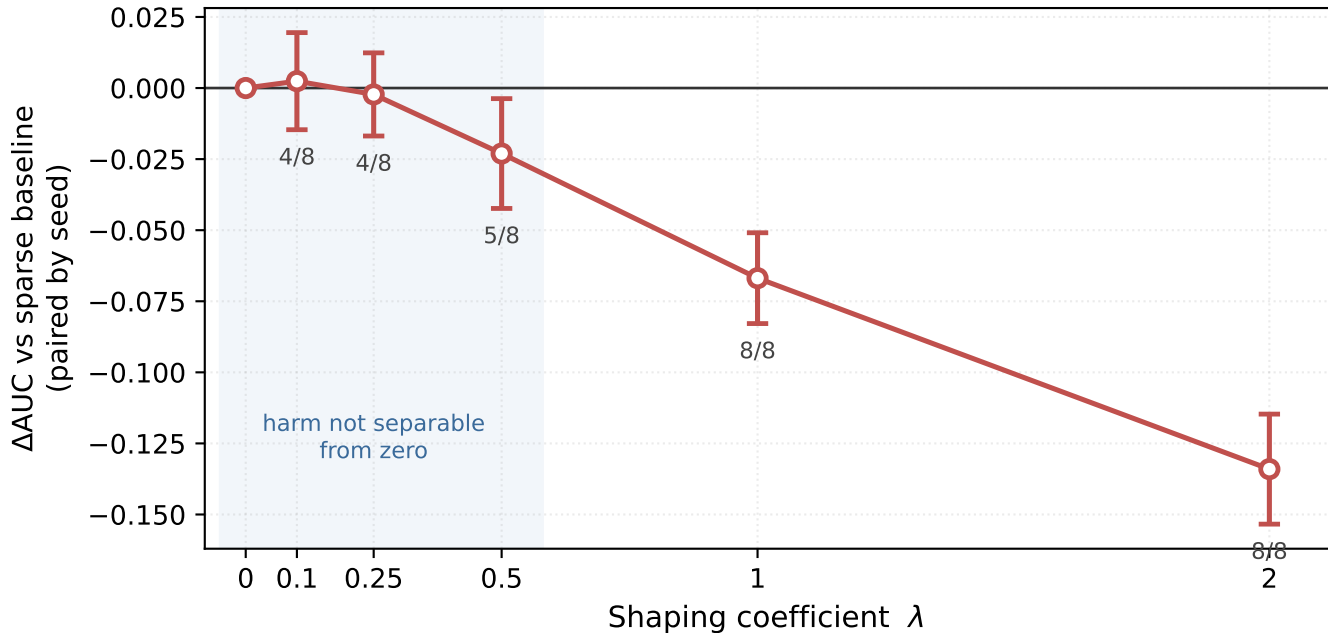
MiniGrid-FourRooms: the harm is controlled by the shaping magnitude ( \lambda = 0 is the baseline by definition; annotations give seeds sharing the sign)
