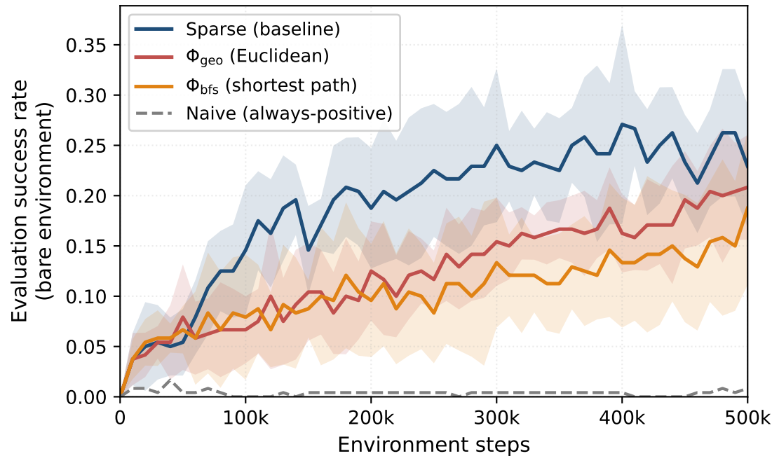
Partial observation (7×7 egocentric view only)
