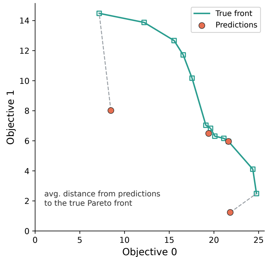
(c) Generational distance
