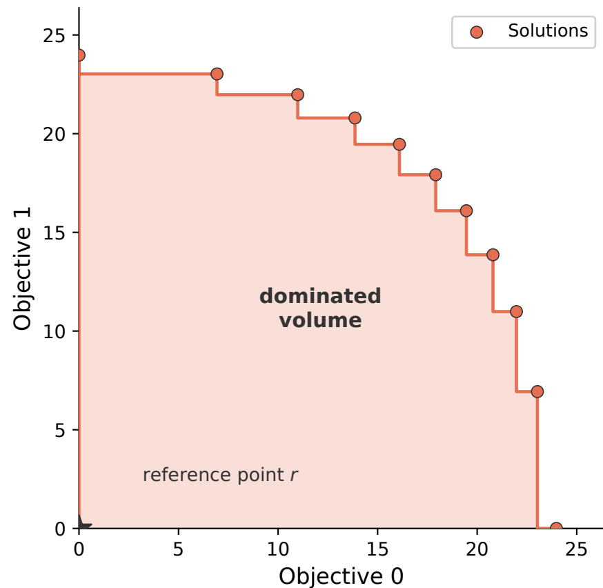
(a) Hypervolume
