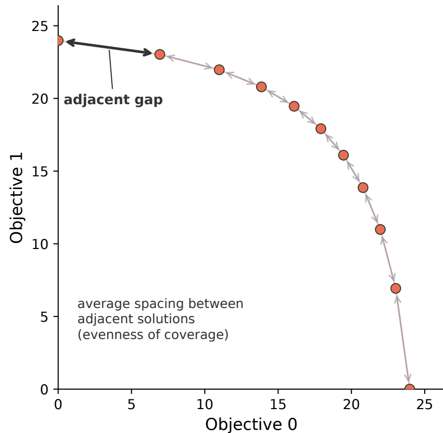
(b) Sparsity
