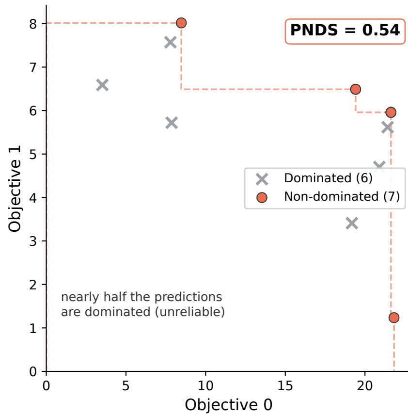
(b) Non-dominated %
