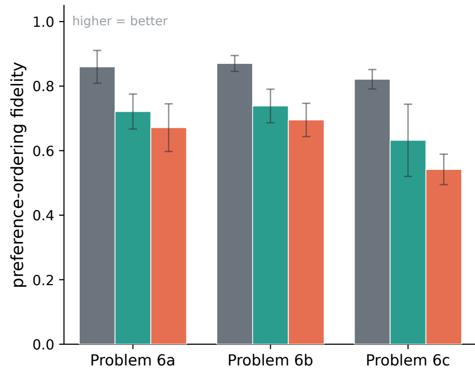
(c) Ordering score
