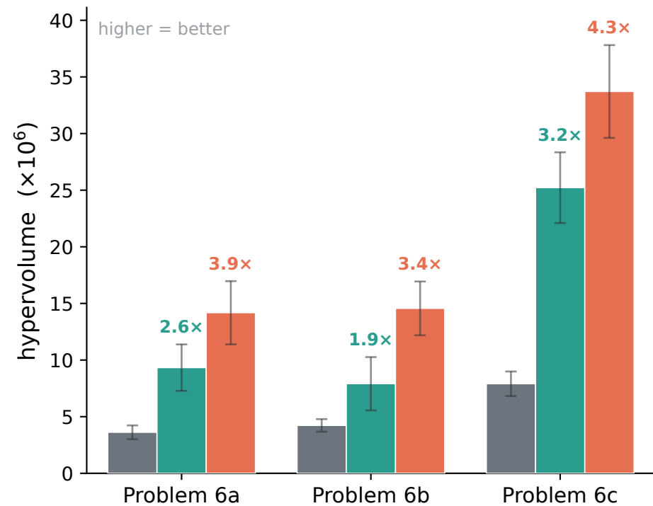
(a) Hypervolume
