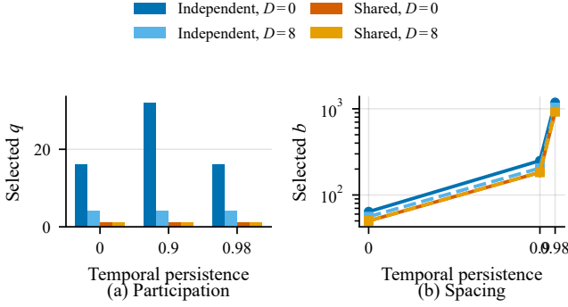
Fig. 2. Joint actions selected by the finite-time Lyapunov certificate in EXP-010B. The left panel reports participation and the right panel reports Markov spacing.
