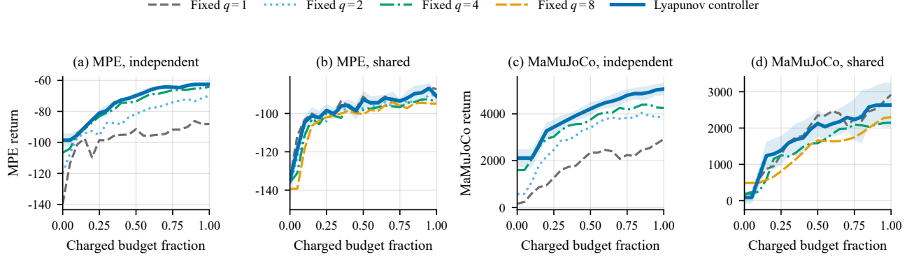
Fig. 5. Fully charged MAPPO team-return learning curves on two cooperative environments with fixed q \in \{1, 2, 4, 8\} and the Lyapunov probe-then-commit controller (eight held-out seeds per regime; shaded bands are controller 95 percent confidence intervals). The controller selects q = 8 for independent streams in both environments, q = 1 for shared MPE streams, and q = 2 for shared MaMuJoCo streams.
