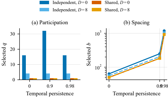
Fig. 2. Joint actions selected by the finite-time Lyapunov certificate in EXP-010B. The left panel reports participation and the right panel reports Markov spacing.
